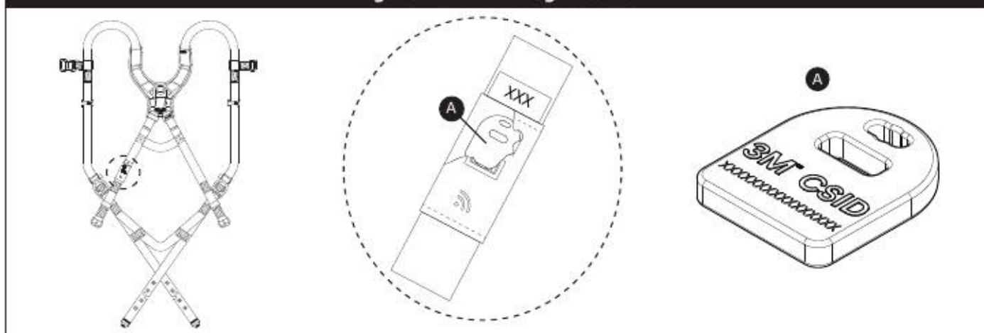
Figure 14 - RFID Tag Location
