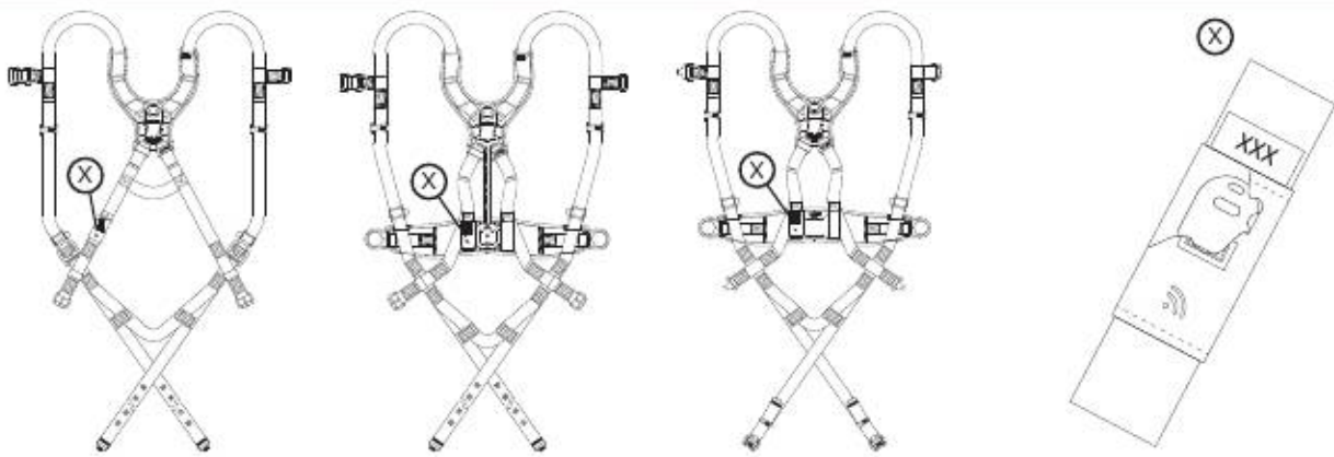
Figure 15 - Product Labels
