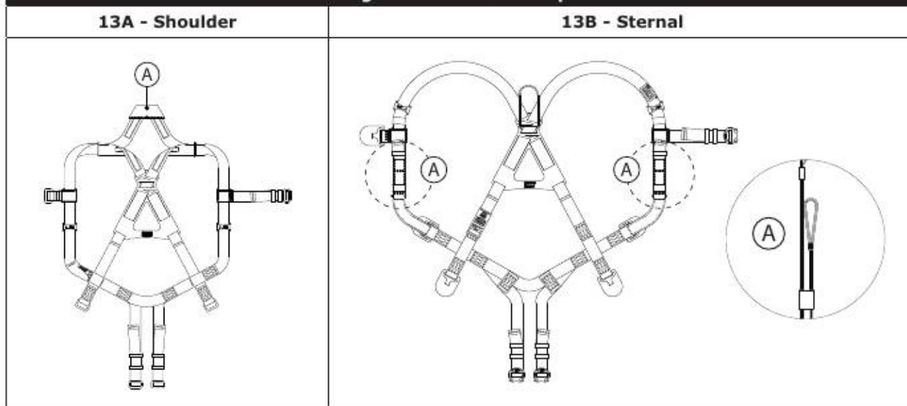
Figure 13 - Rescue Loops
