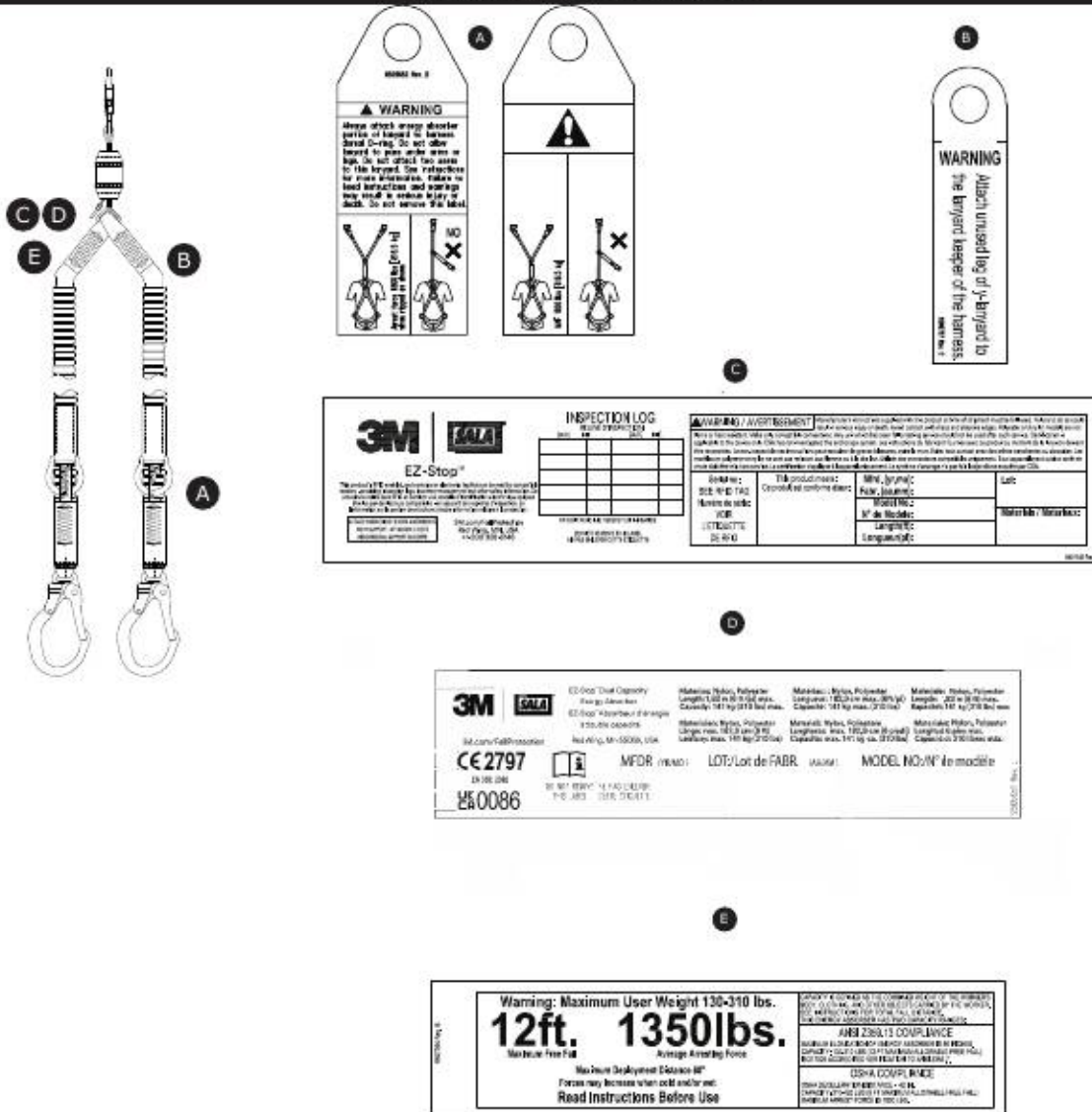
Figure 14 - Product Labels
