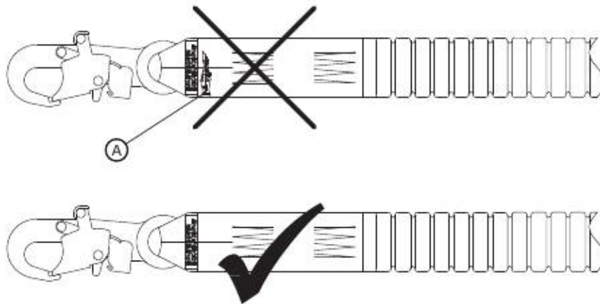
Figure 18 - Impact Indicator Inspection
