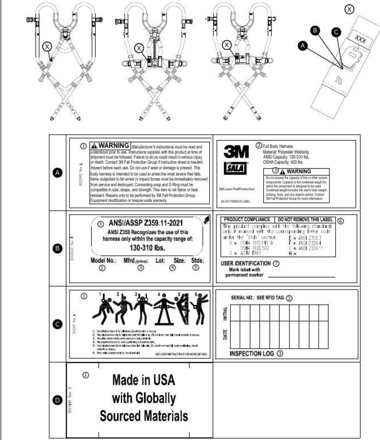
Figure 20 - Product Labels
