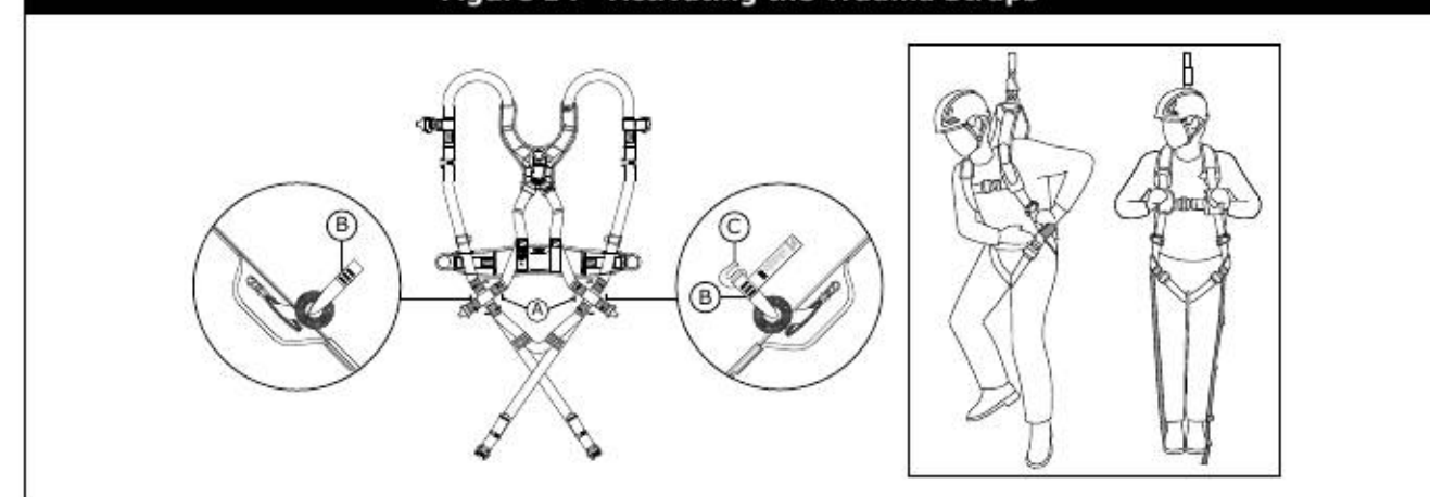
Figure 14 - Activating the Trauma Straps
