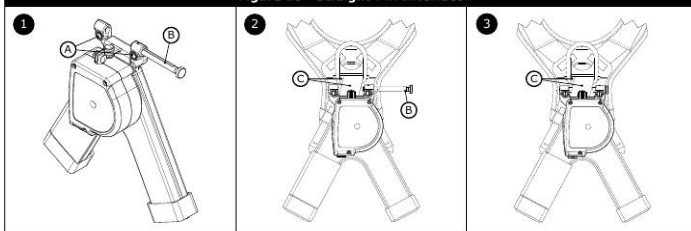
Figure 10 - Straight-Pin Interface
