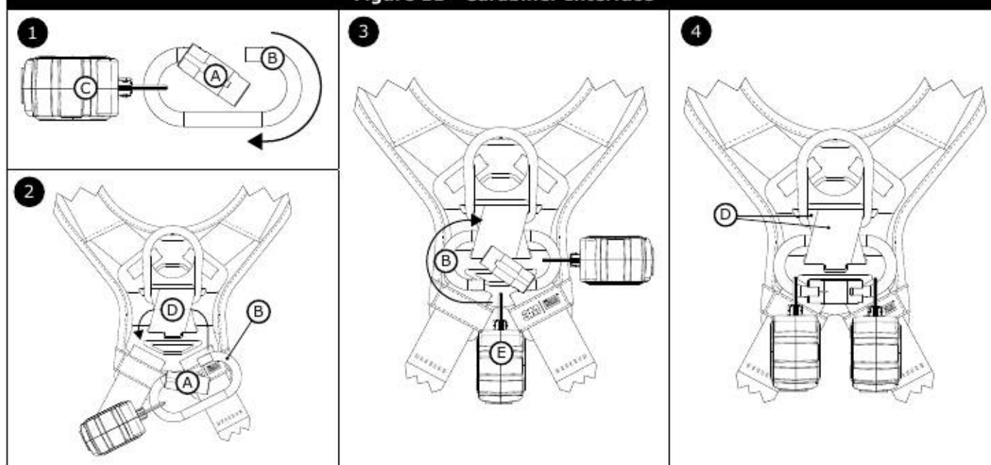
Figure 11 - Carabiner Interface
