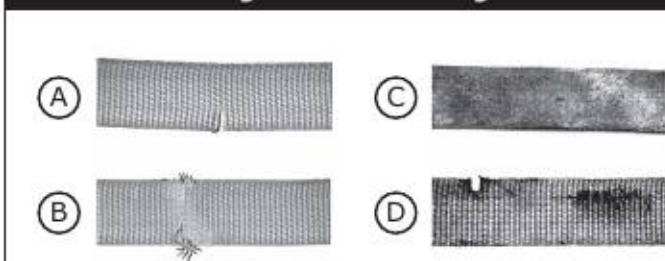
Figure 21 - Webbing
