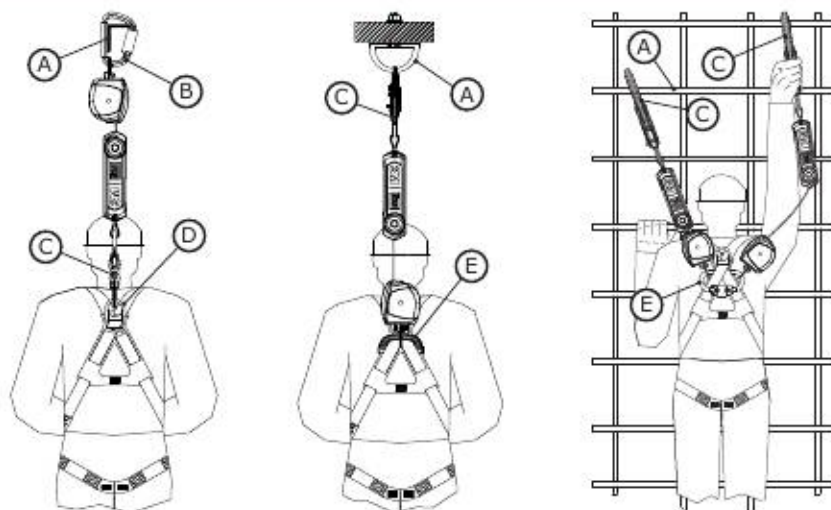
Figure 7 - Connecting to Anchorage
