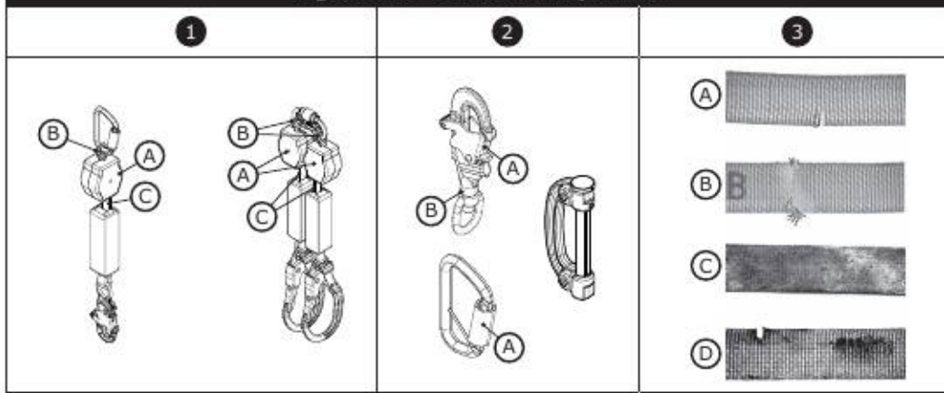
Figure 13 - Energy Absorber Inspection
