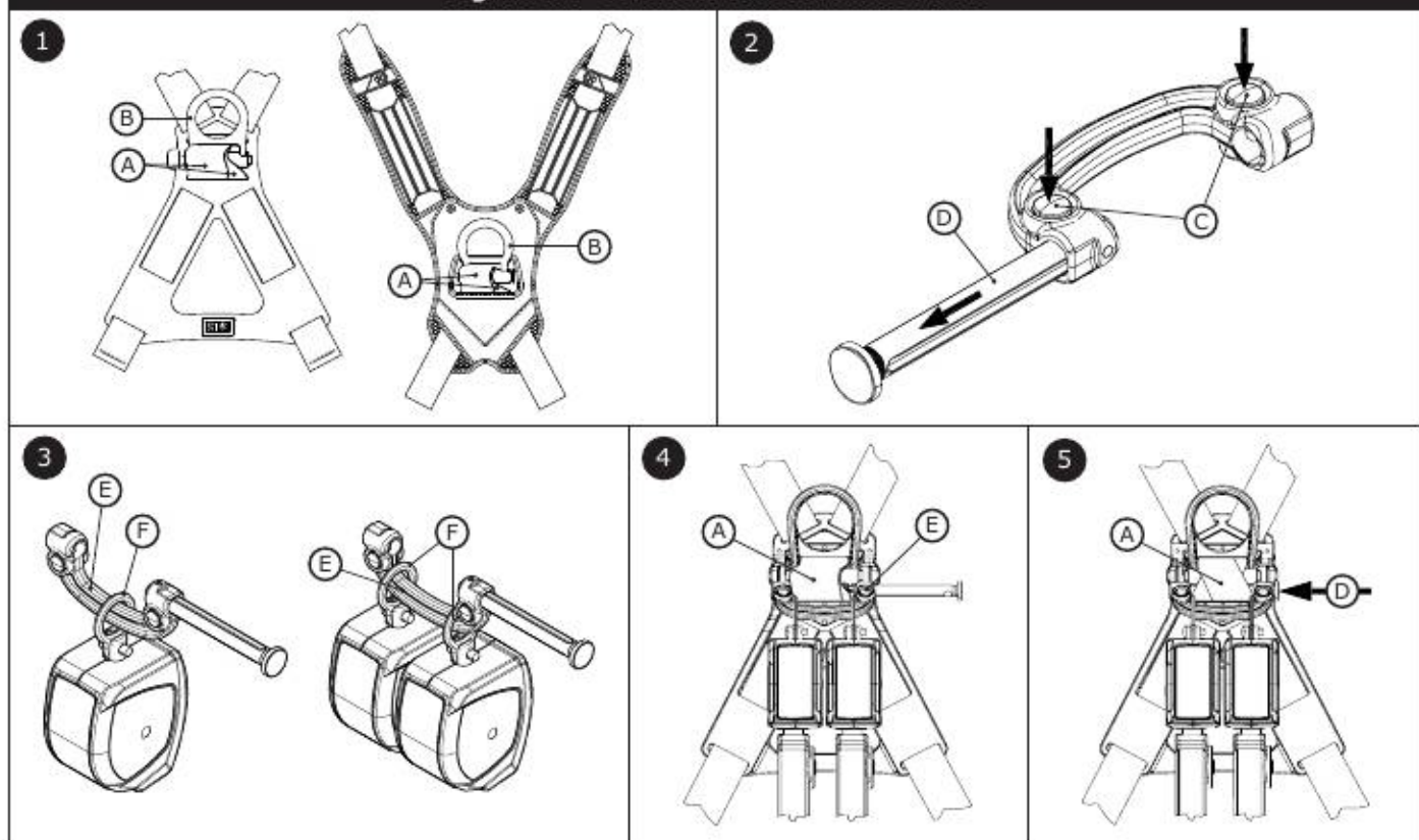
Figure 8A - Standard Harness Interface
