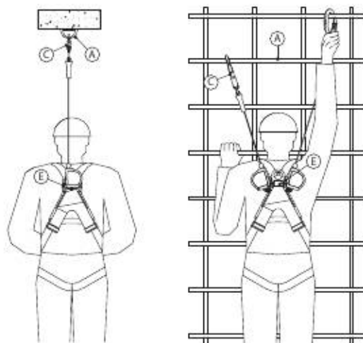
Figure 7 - Connecting to Anchorage
