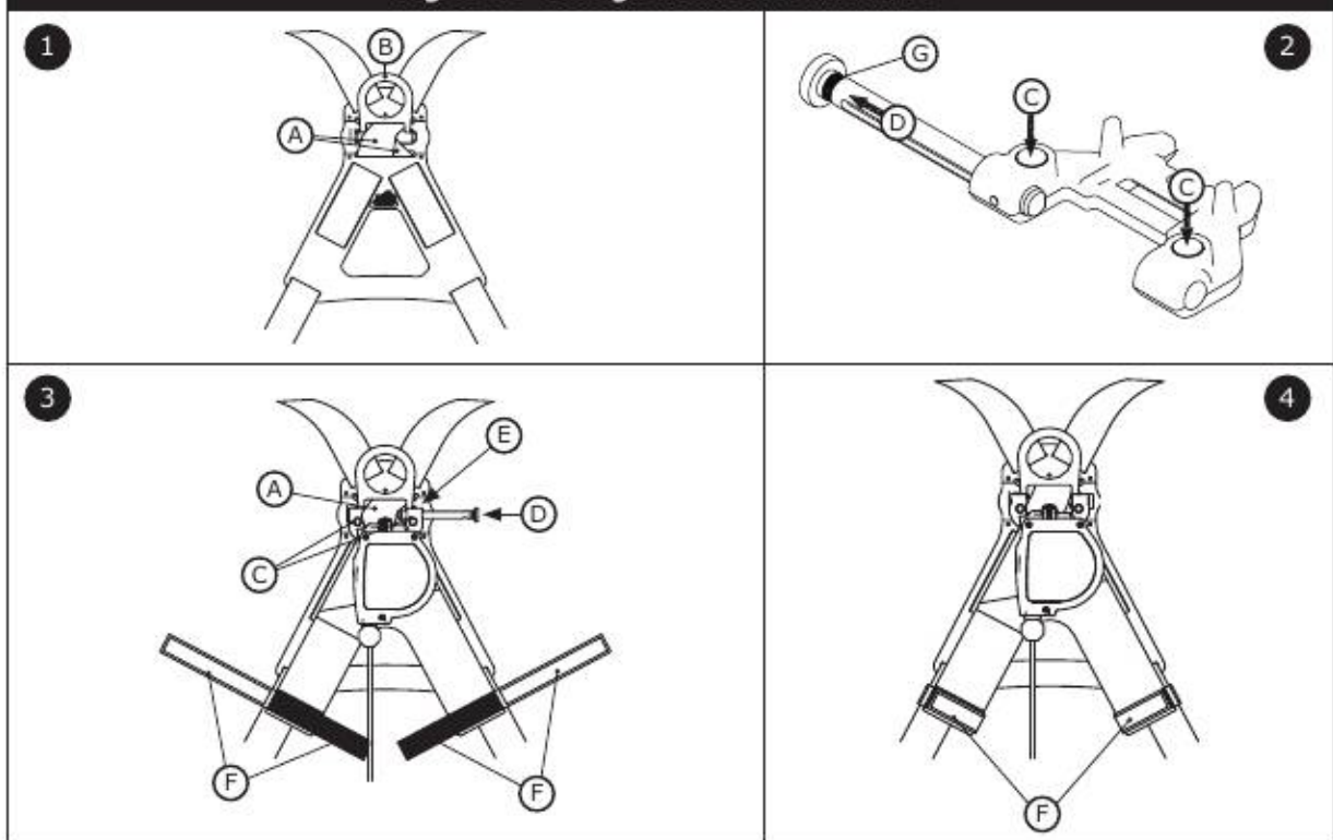
Figure 8 - Integral Harness Interface
