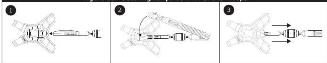
Figure 10 - Securing Lanyards with Choker Loops
