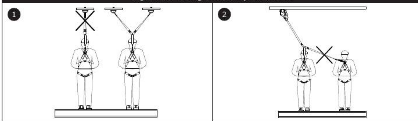
Figure 13 - Using Twin-Lanyard Models
