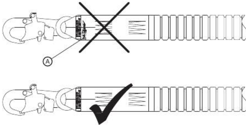
Figure 20 - Impact Indicator Inspection
