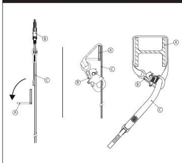
Figure 11 - Tie-Back Connections: Tie-Back Connector
