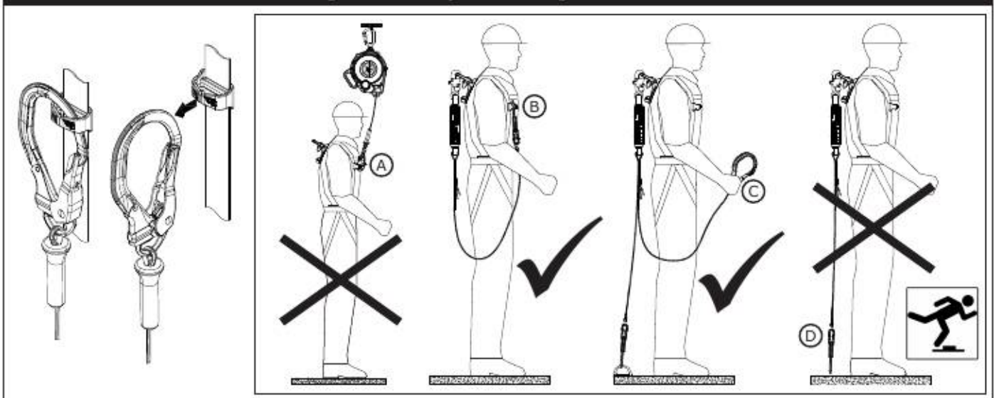
Figure 6 – Lanyard Parking Attachment
