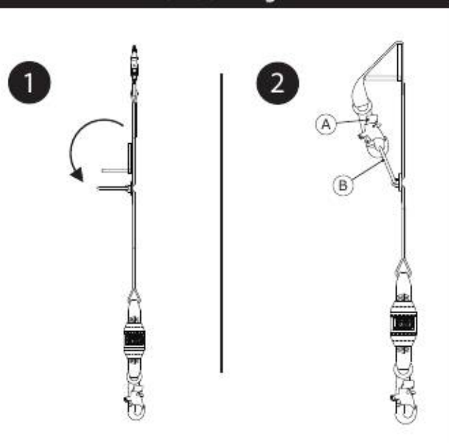
Figure 12 - Tie-Back Connections: Tie-Back Ring
