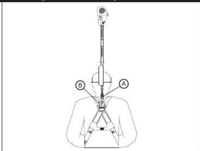
Figure 9 - Connecting to a Harness
