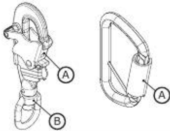
Figure 18 - Connector Inspection
