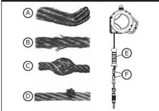
Figure 14 - Wire Rope Lifeline
