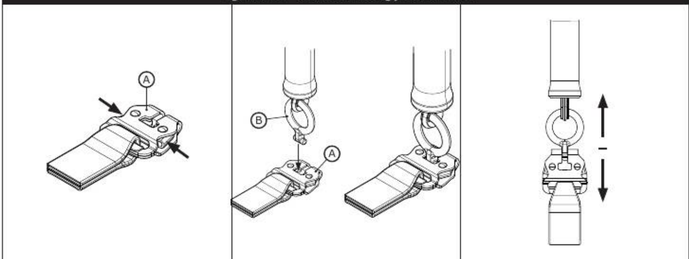
Figure 10 - Modular Energy Absorbers
