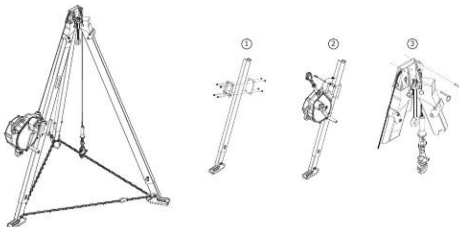
Figure 9 - Tripod Mounting
