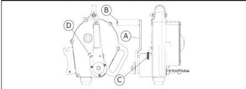
Figure 16 - SRD-R Inspection
