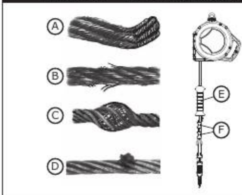
Figure 14 - Wire Rope Lifeline
