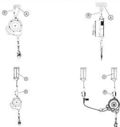
Figure 7 - Connecting to Anchorage
