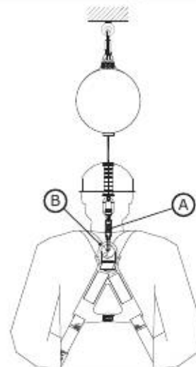
Figure 8 - Connecting to a Harness
