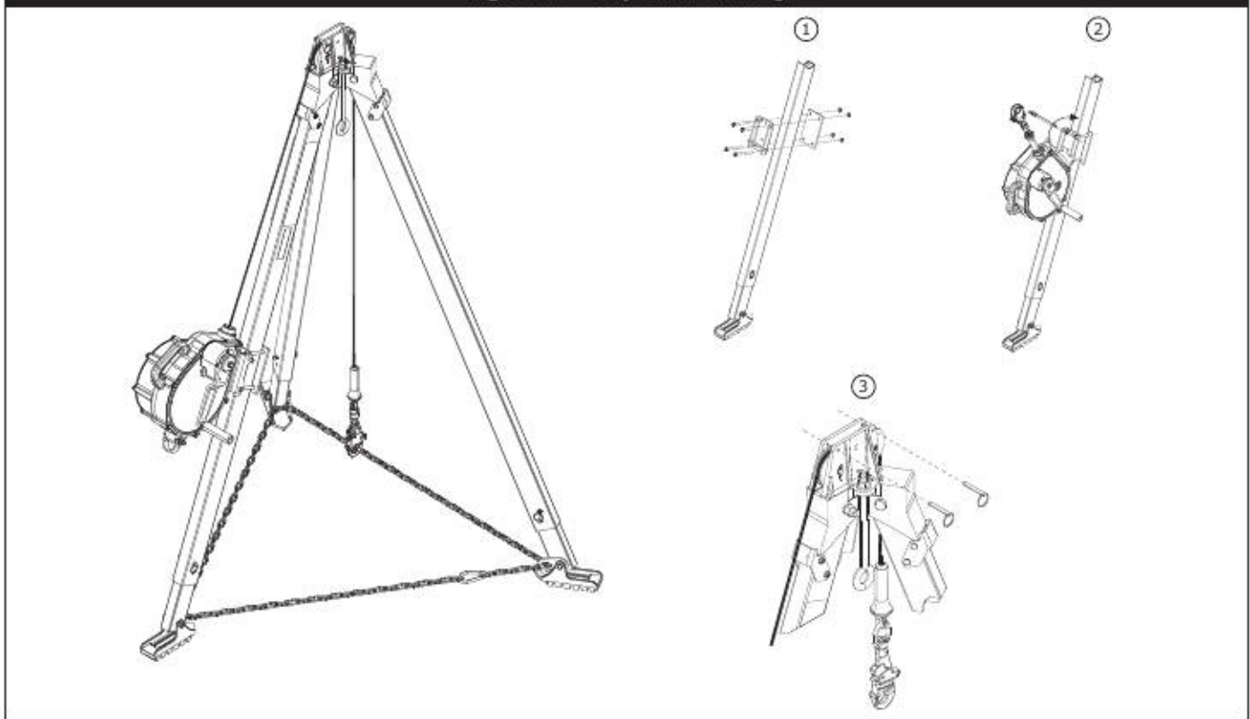
Figure 9 - Tripod Mounting
