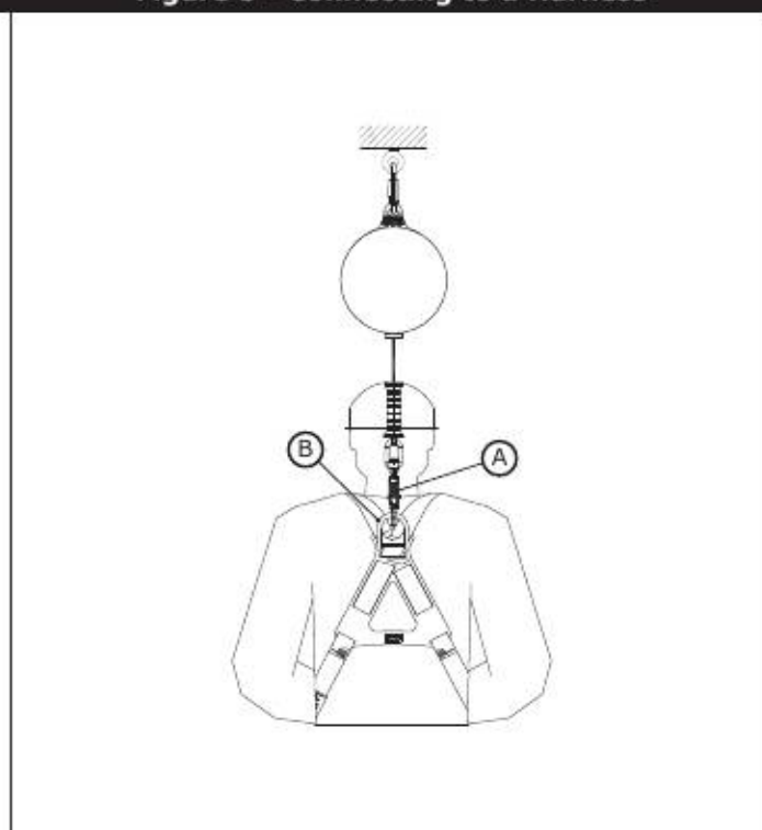
Figure 8 - Connecting to a Harness
