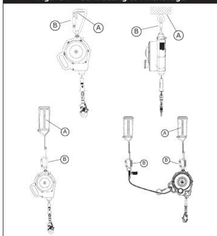
Figure 7 - Connecting to Anchorage
