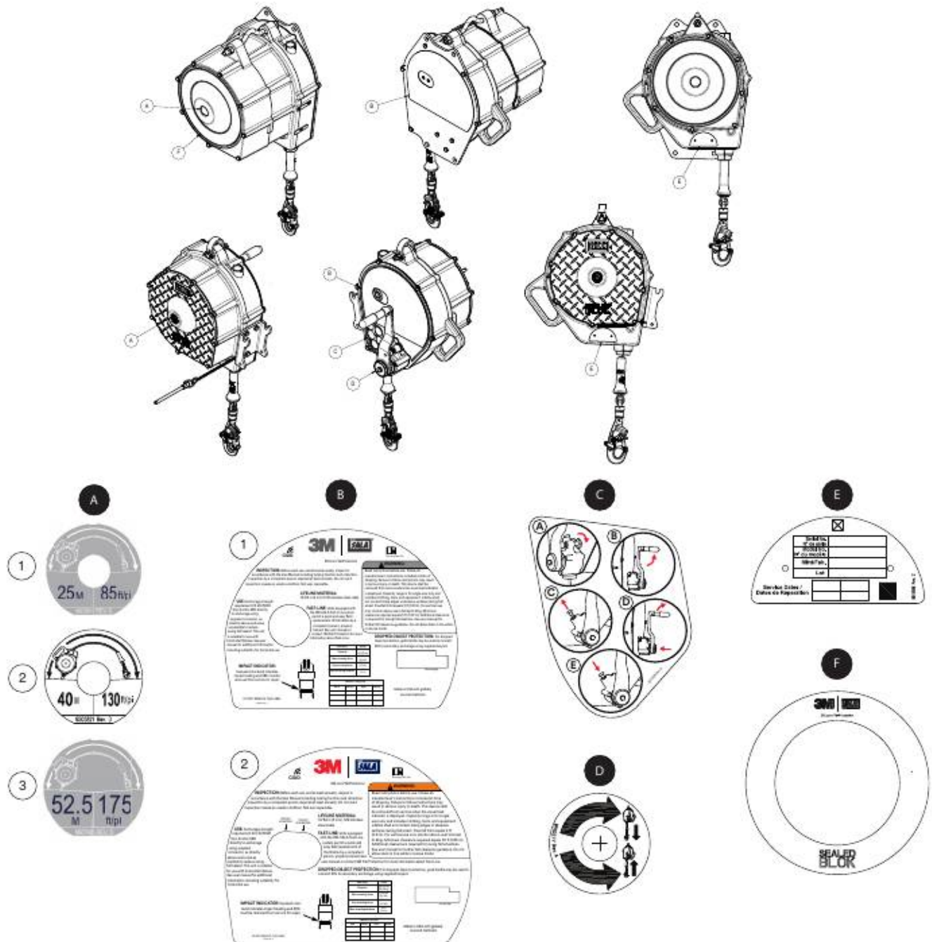
Figure 12 - Product Labels
