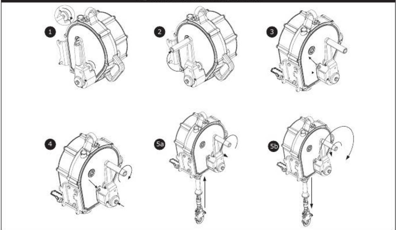
Figure 10 - Retrieval Operation
