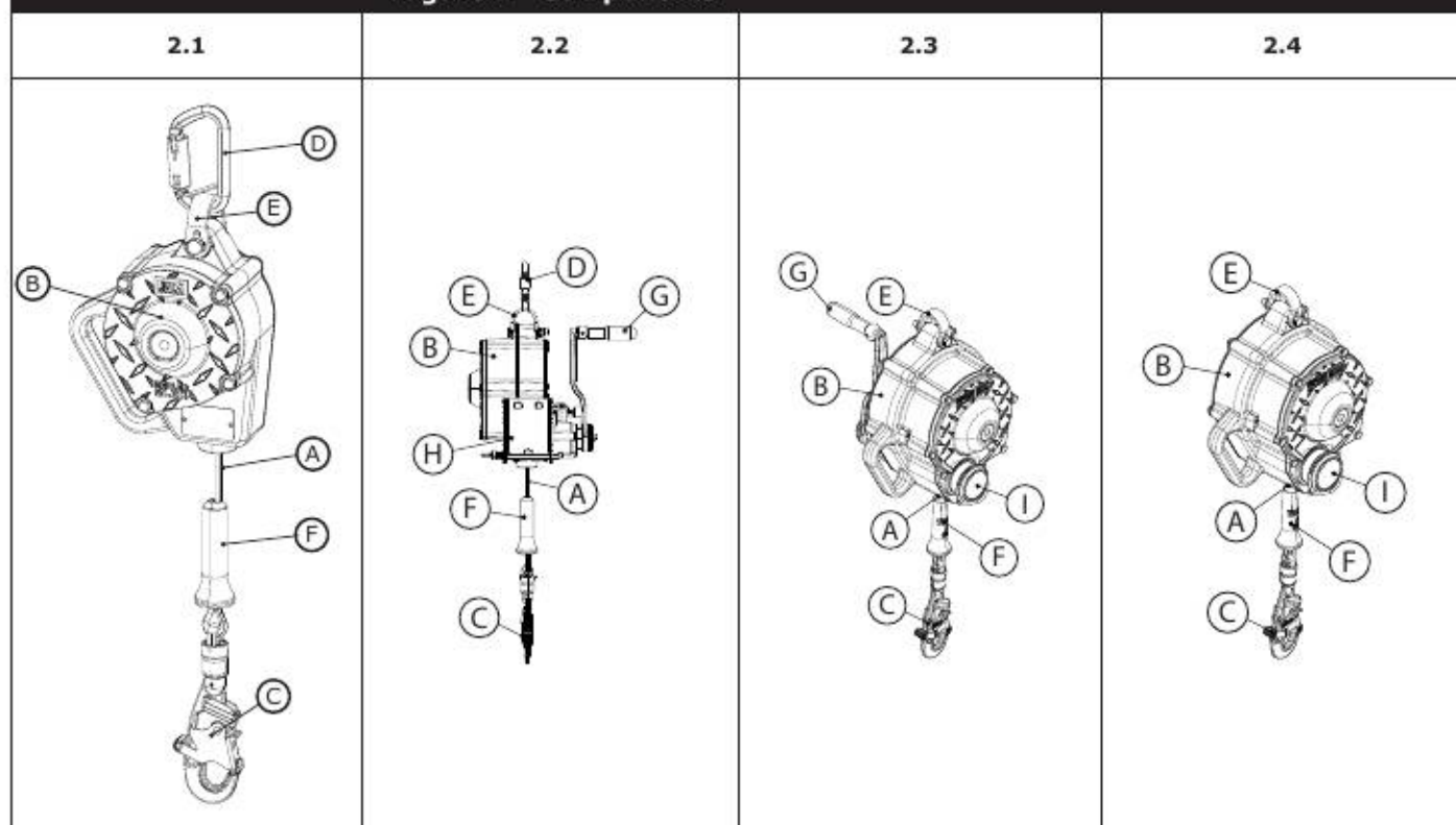
Figure 2 - Components
