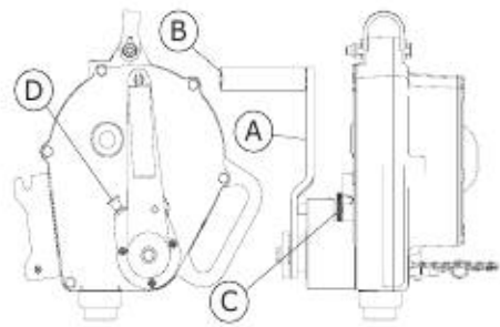
Figure 15 - SRD-R Inspection
