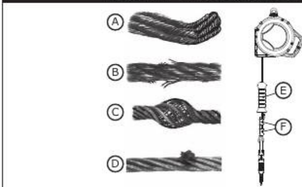
Figure 14 - Wire Rope Lifeline
