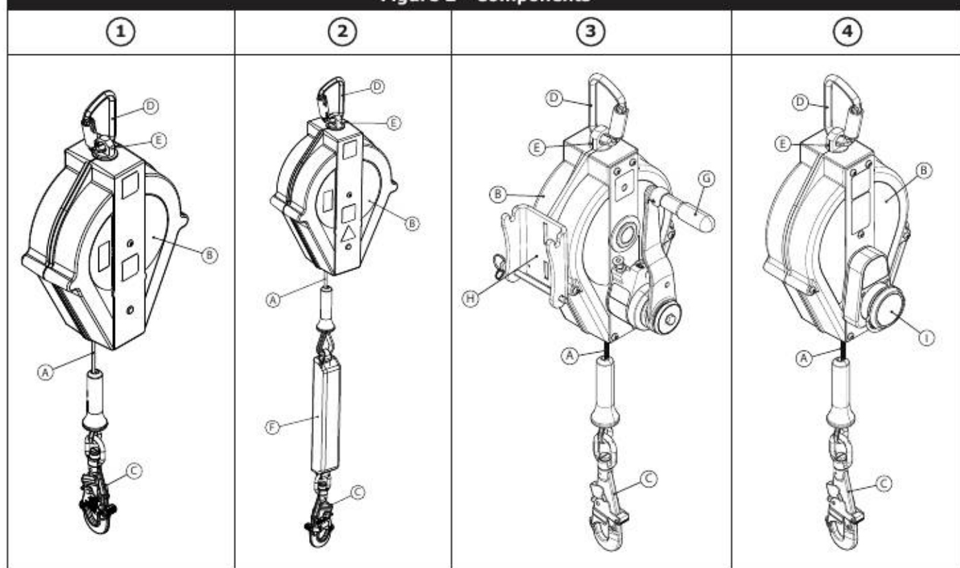
Figure 2 - Components
