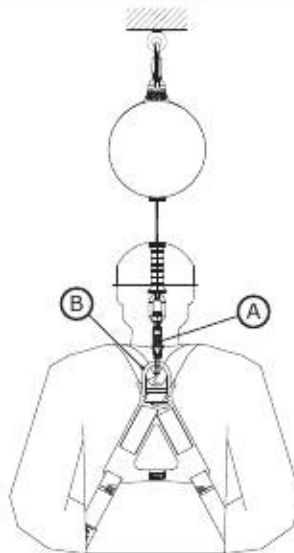
Figure 8 - Connecting to a Harness
