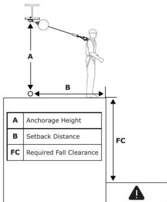
Fall Clearance Chart #1 - 50 ft. (15.2 m) SRD Models
