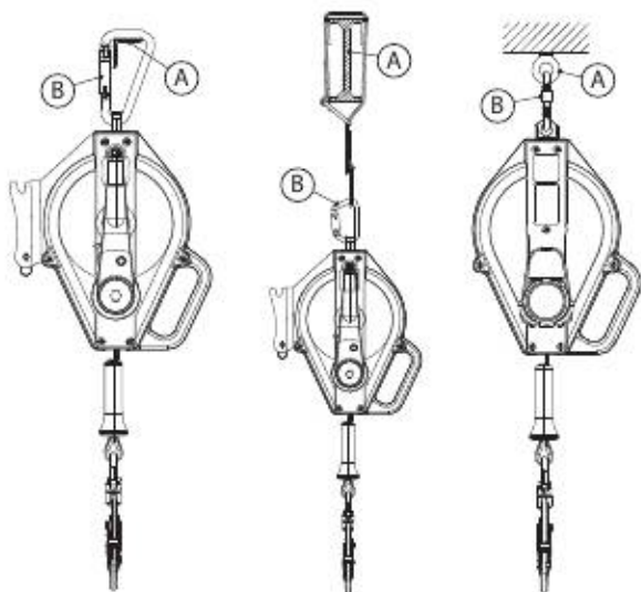
Figure 7 - Connecting to Anchorage
