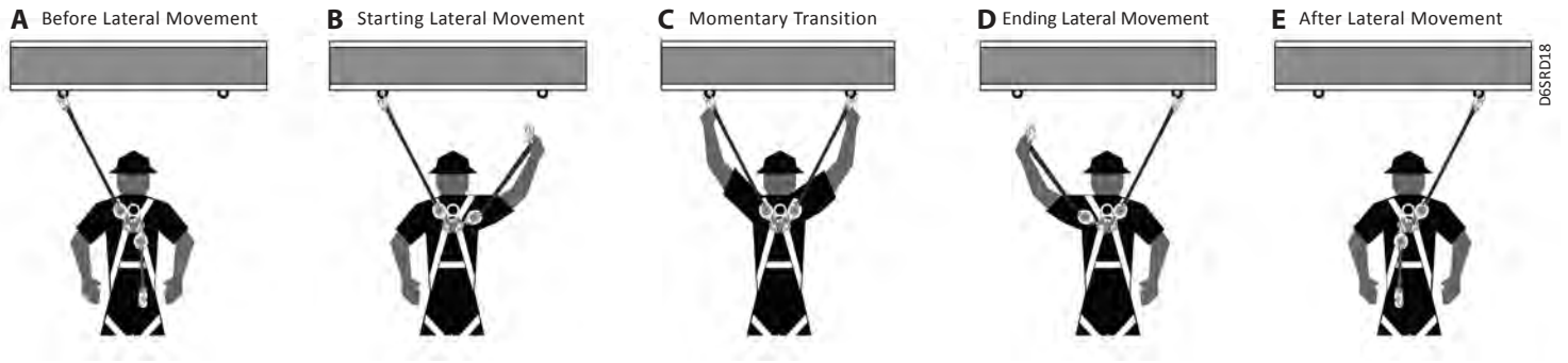
Fig. 7: Use of Twin-leg SRDs for Lateral Movement
