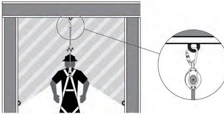
Fig. 2B: SRD Orientation and Acceptable Anchorage Range Single-leg SRD mounted to Anchorage
