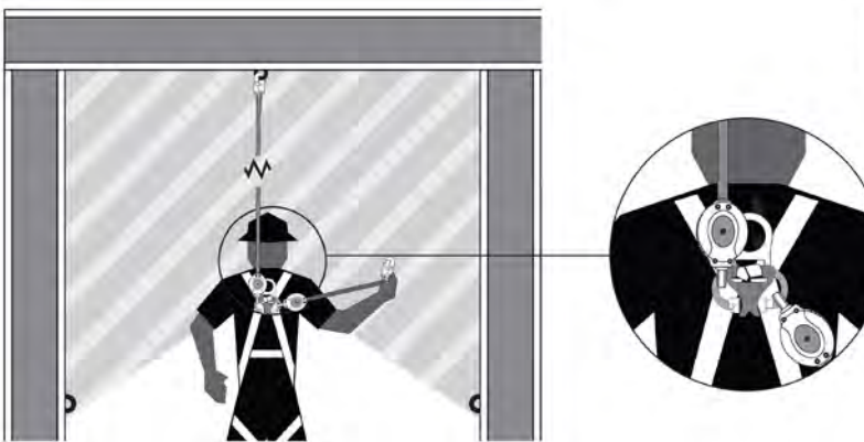
Fig. 2C: SRD Orientation and Acceptable Anchorage Range Twin-leg SRD mounted to Dorsal D-ring
