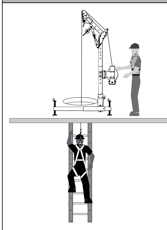
Figure 3 - Single Line 3-Way Only – Entry/Egress using ladder
