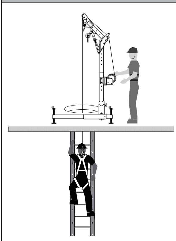
Figure 2 - Single Line Winch Only – Entry/Egress Using Ladder
