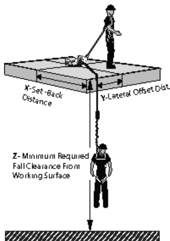
Chart 2 - 30' FT-R+ MRFC Non-Overhead Anchorage for 130 to 310 lbs. (59 to 141 kg) Users
