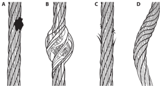
Figure 6: Inspection of Cable
