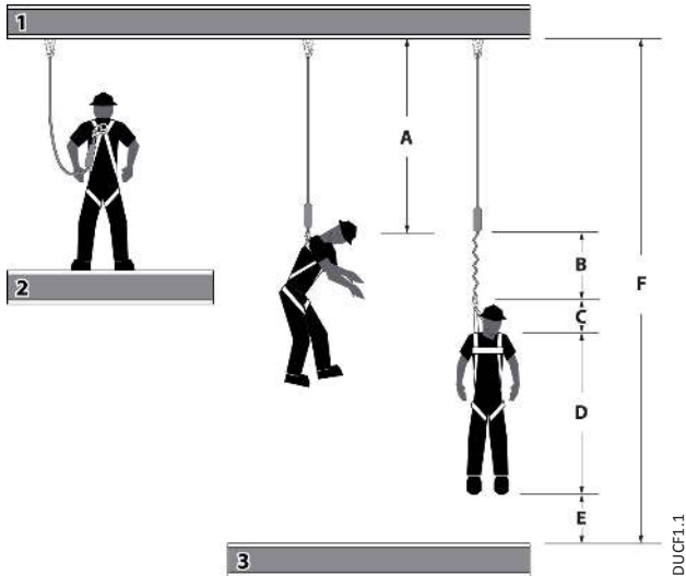
Fig. 1 - Minimum Clear Fall Requirement: 6 ft Shock Absorbing Lanyard Measured from Overhead Anchorage Connector
