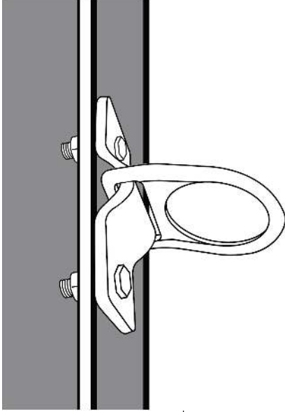
Figure 8: Bolt-on Installation Type A
