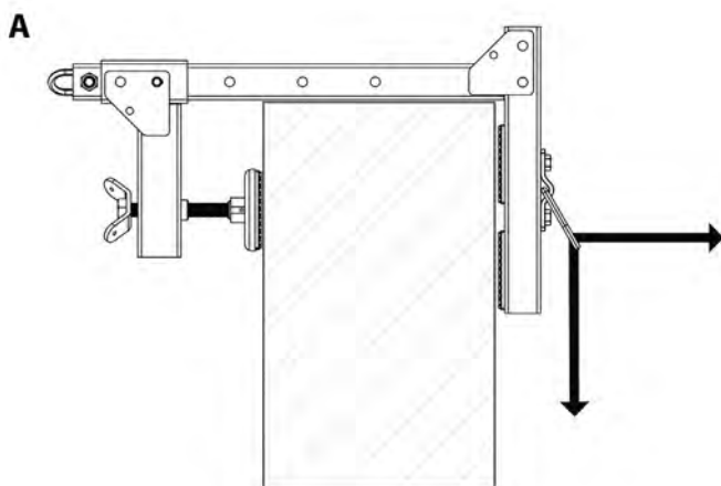
Fig. 4: Load Direction and Working Range
