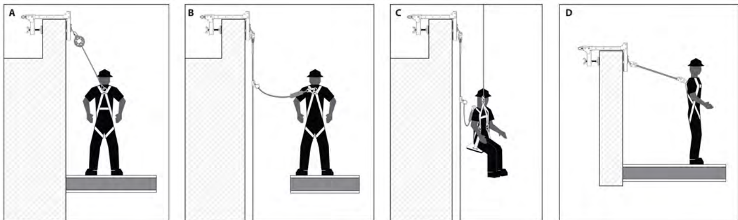
Fig. 2: Fall Protection Uses with a Parapet Anchor
