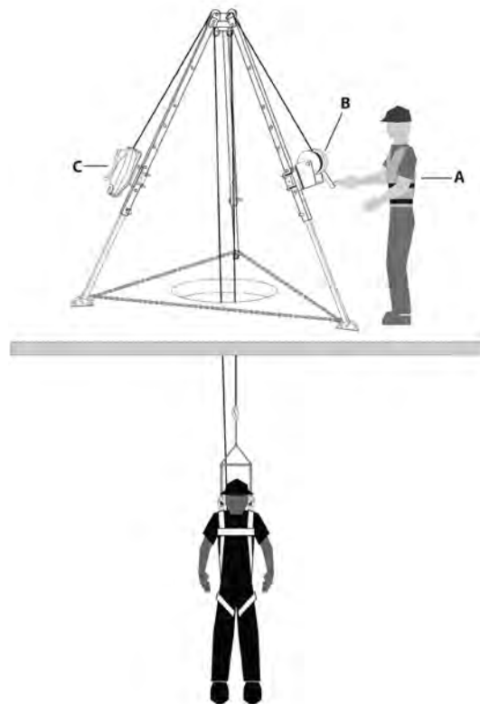
Figure 2C: Tripod Use with Winch and 3-Way SRL-R
