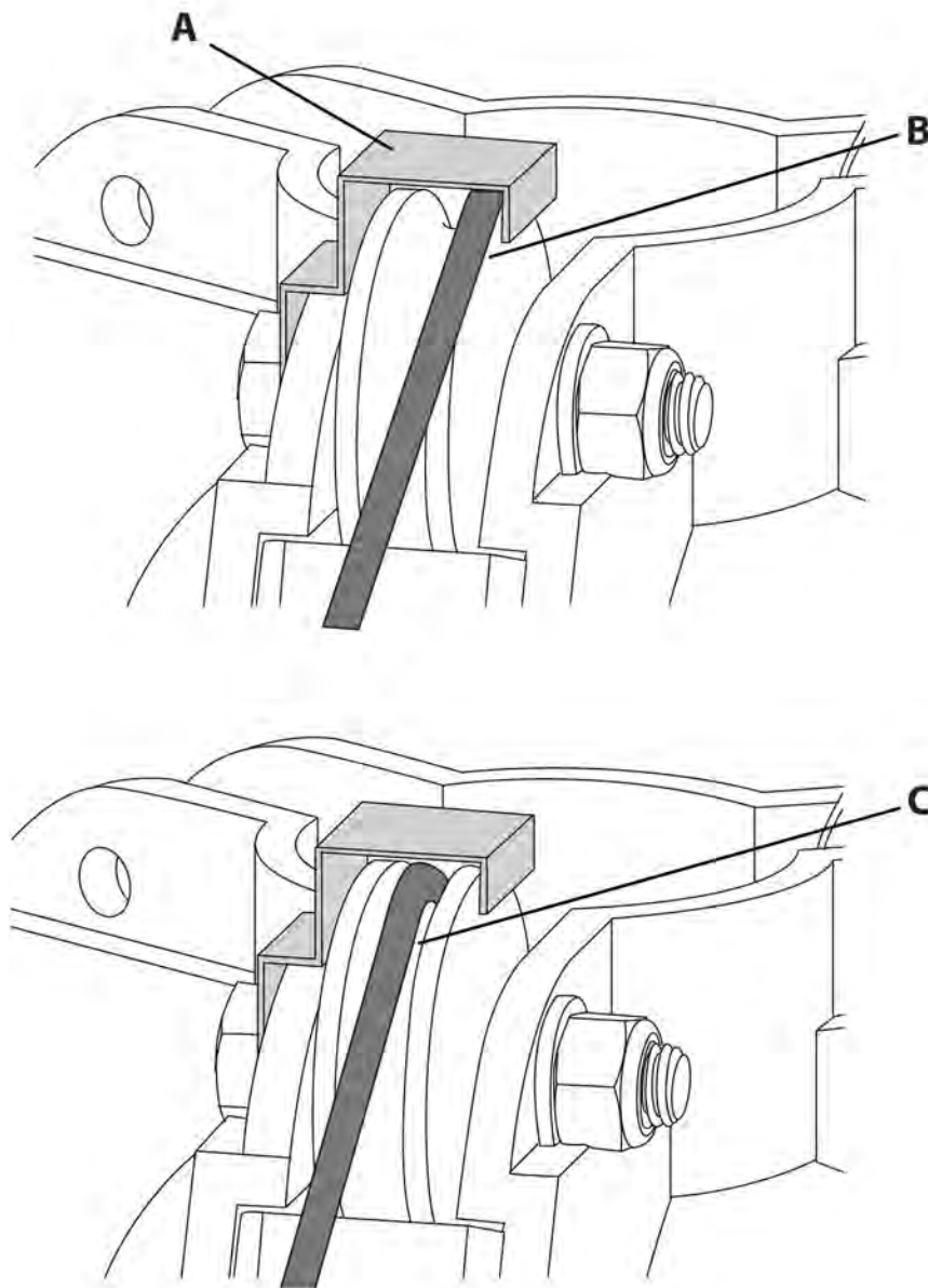
Figure 6: Integral Pulley Use
