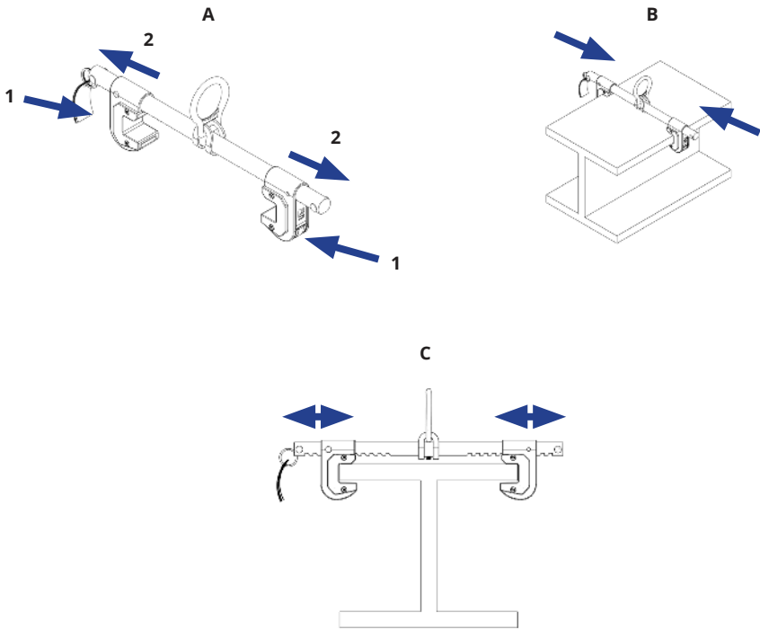
Figure 4 - Installation Instructions
