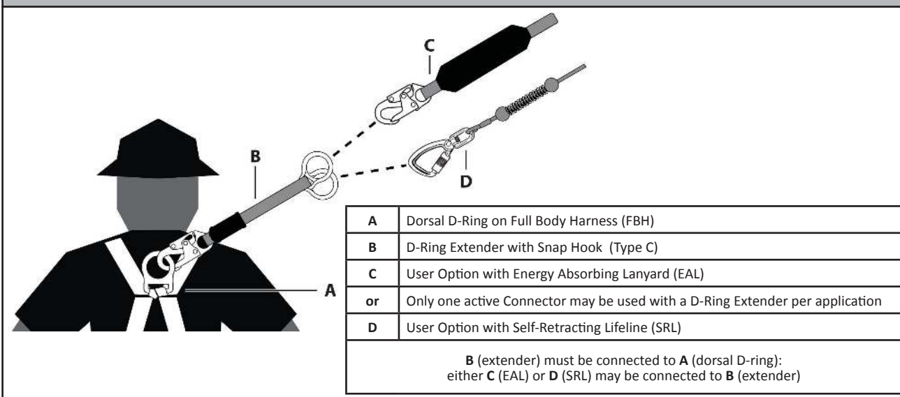
Figure 9: Suitable Use of D-Ring Extender Type C
