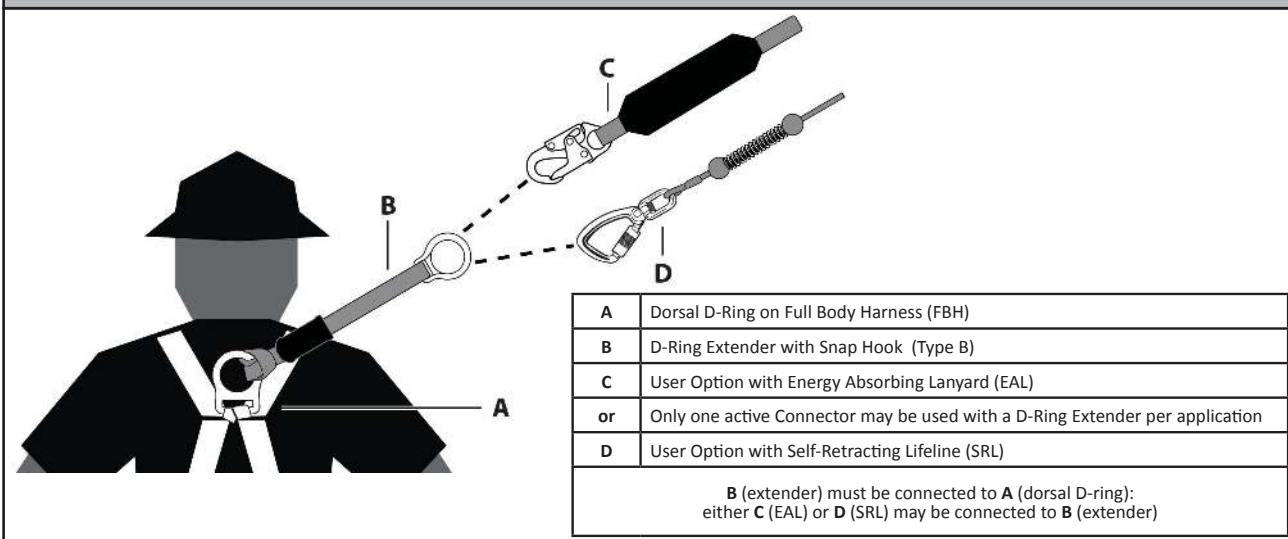
Figure 8: Suitable Use of D-Ring Extender Type B
