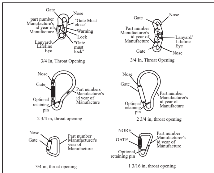
SNAP HOOKS & CARABINERS
