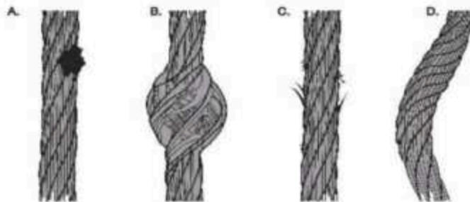
Drawing 3.
