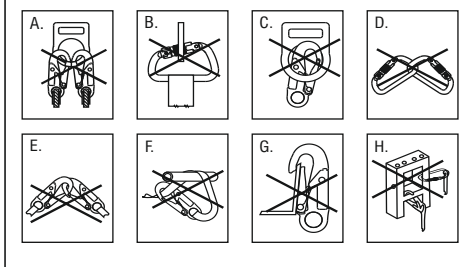
Fig. 3 - Inappropriate Connections
