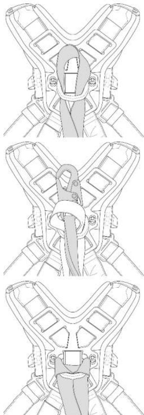
Figure 3 Hitchloop Connection
