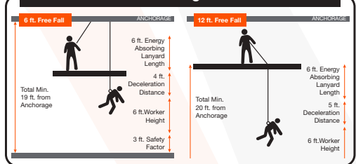
Illustration 3: Calculating Total Fall Distance
