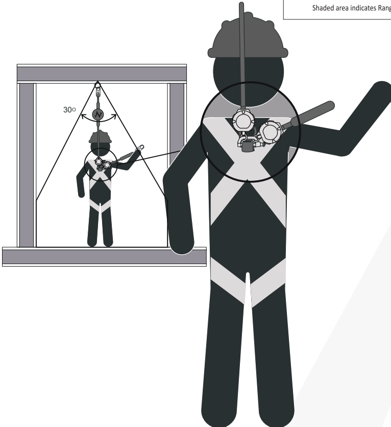
Figure 3C: Pygmy Hog SRD Orientation and Acceptable Anchorage Range
