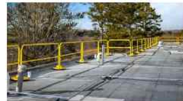
Free Standing Guardrail System
