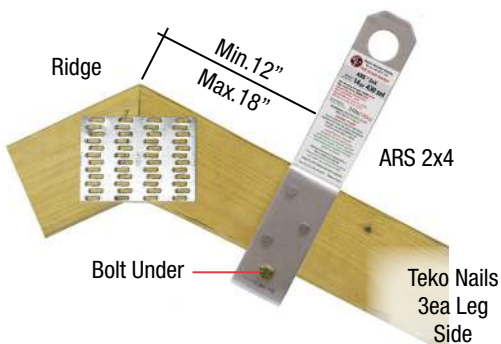
Fig.5 2x4 Top Chord
