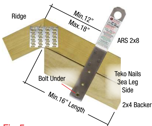
Fig.5 2x4 Top Chord
