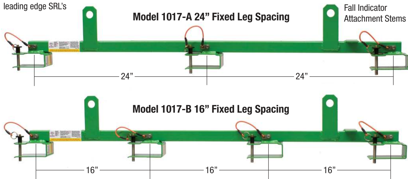
1-1/2"x1-1/2"x1/8" Cross-bar
