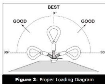
Figure 2: Proper Loading Diagram
