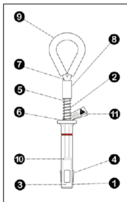
Figure 1: Key components of removable concrete anchor
