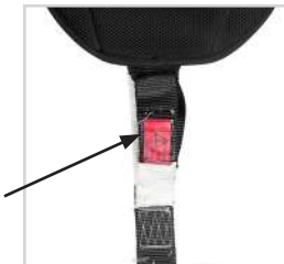
Red Exposed - Impact Indicator Broken - Remove From Service -
