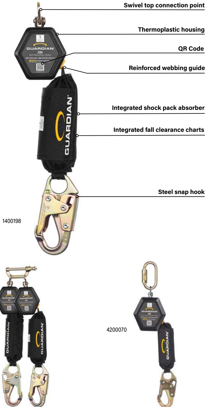
Steel snap hook
